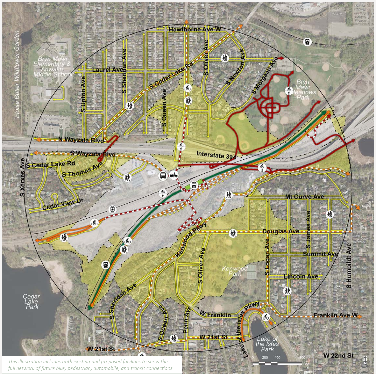
FIGURE 4-9. ACCESS + CIRCULATION PLAN
